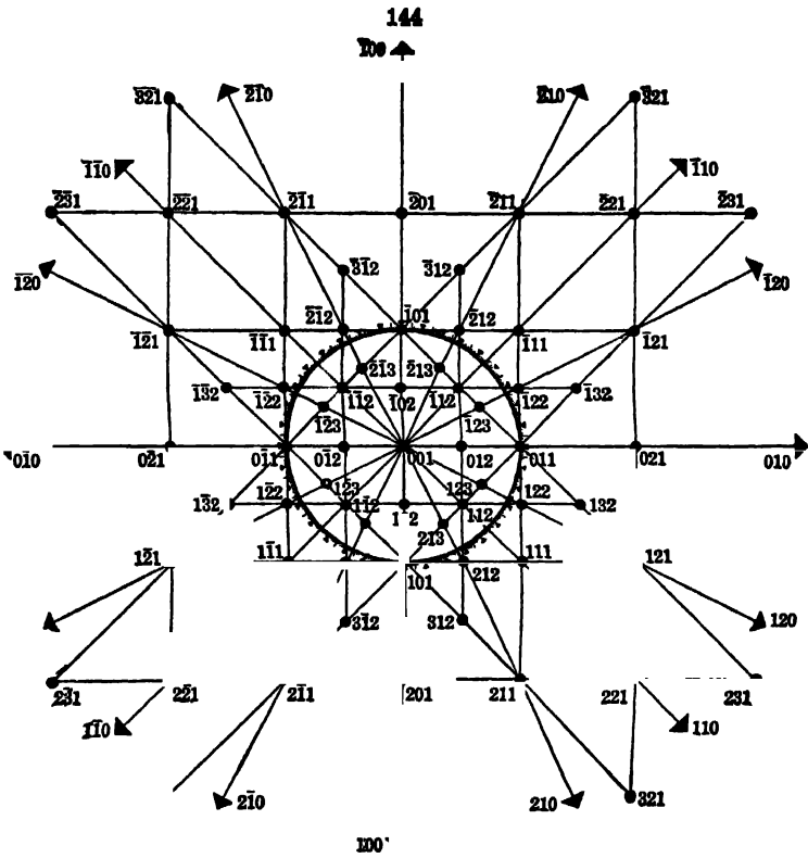
Gnomonic Projection of Isometric Forms (Cube (100), Octahedron (111), Dodecahedron (110), Tetrahexahedron (210), Trisectahedron (221), Trapezohedron (211), Hexooctahedron (321))
